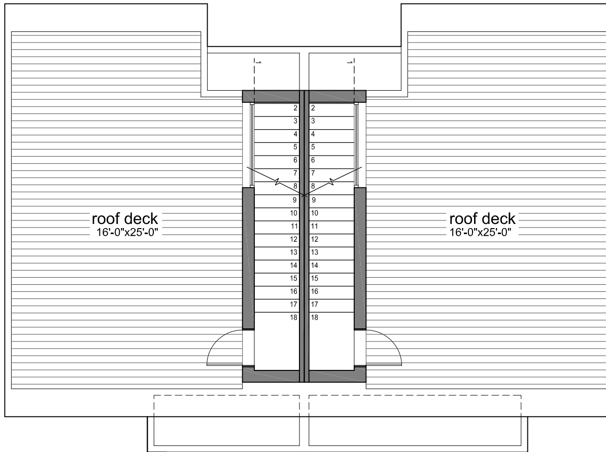
roof plan
