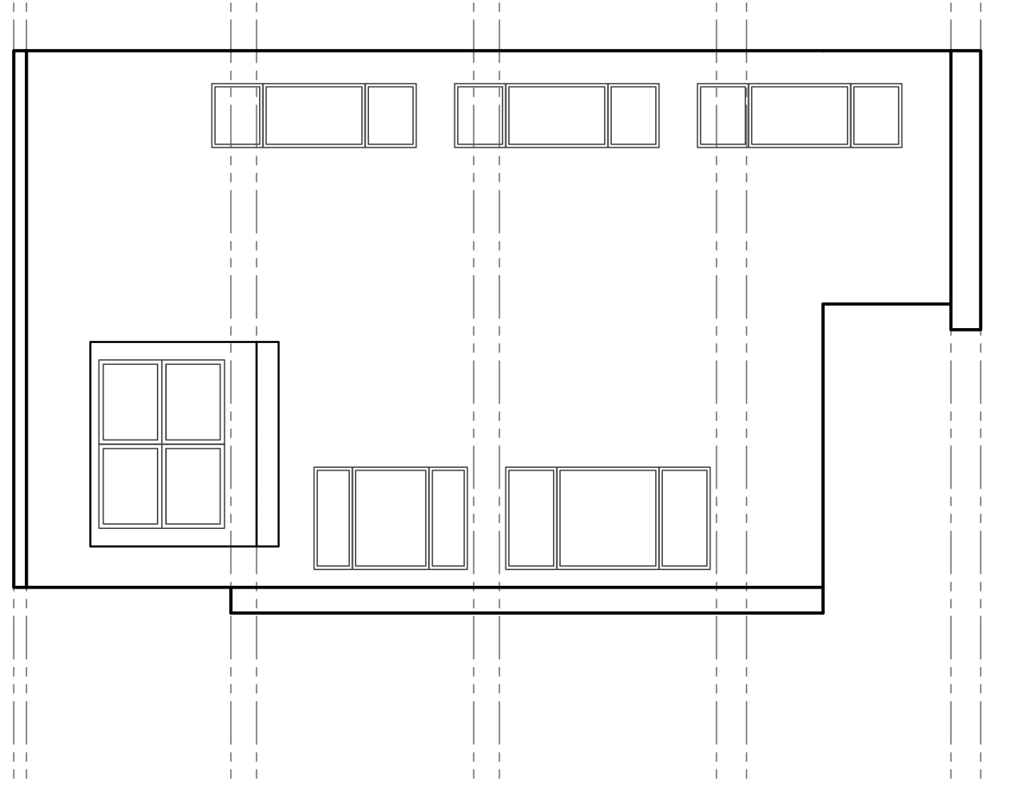
NORTH SCALE: 3/16" = 1'-0"
