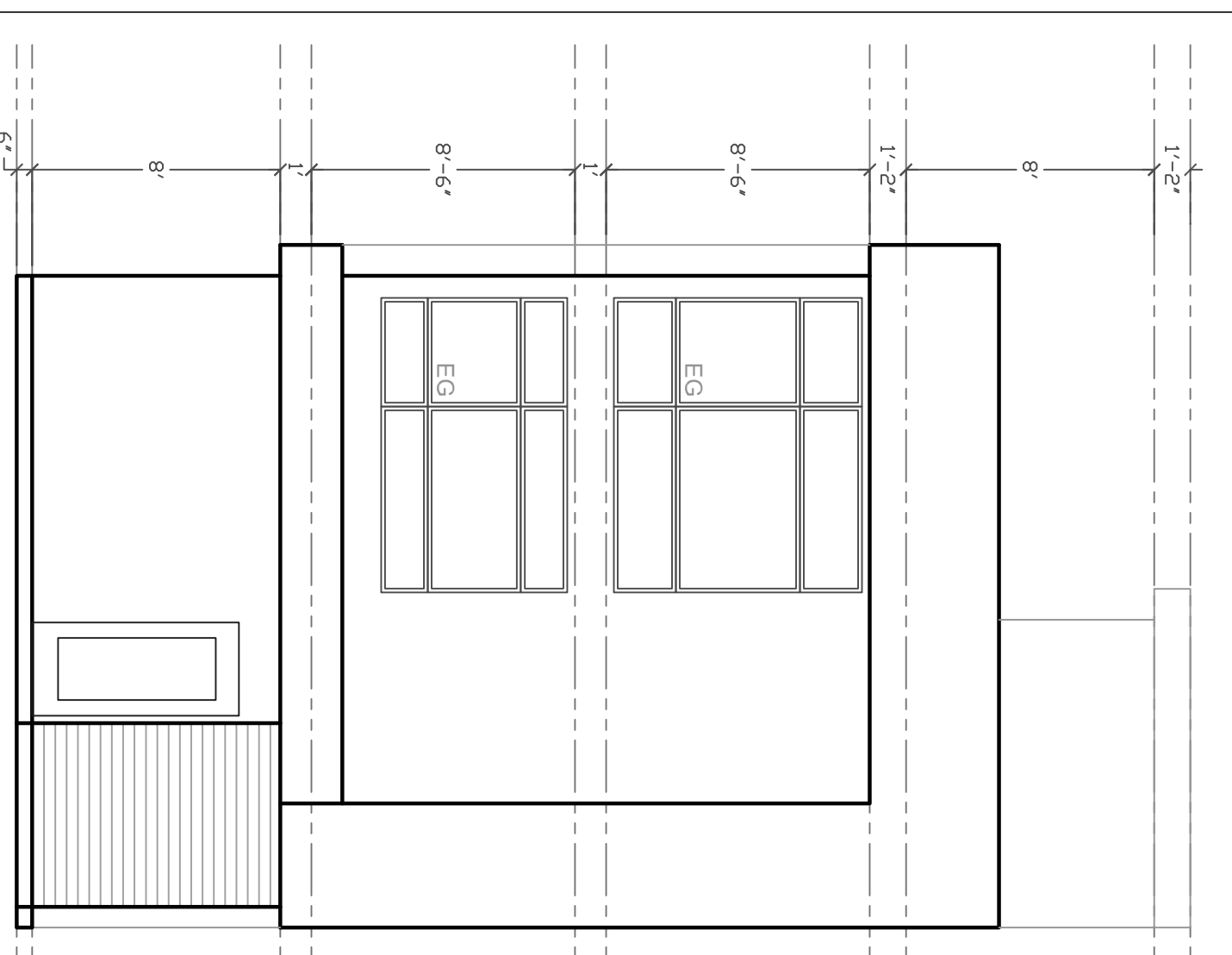
SOUTH SCALE: 3/16" = 1'-0"
