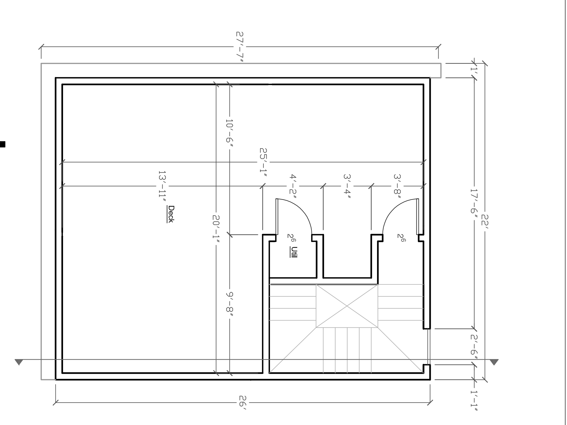
ROOF SCALE: 1/4" = 1'-0"
