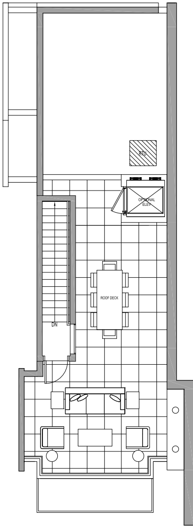
ROOF DECK
