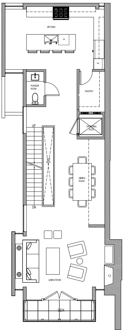
THIRD FLOOR
