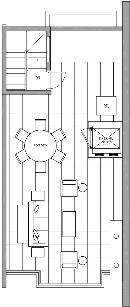
ROOF DECK
